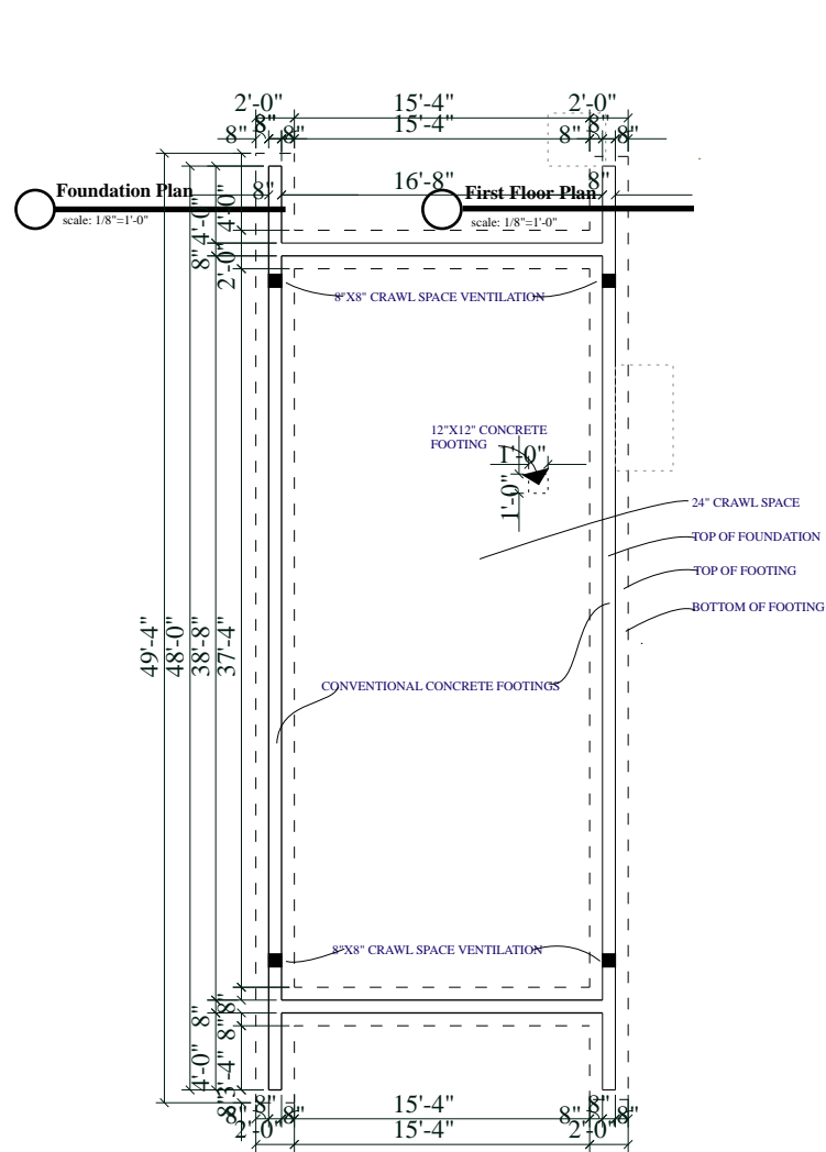
Foundation Plan scale: 1/8"=1'-0"
